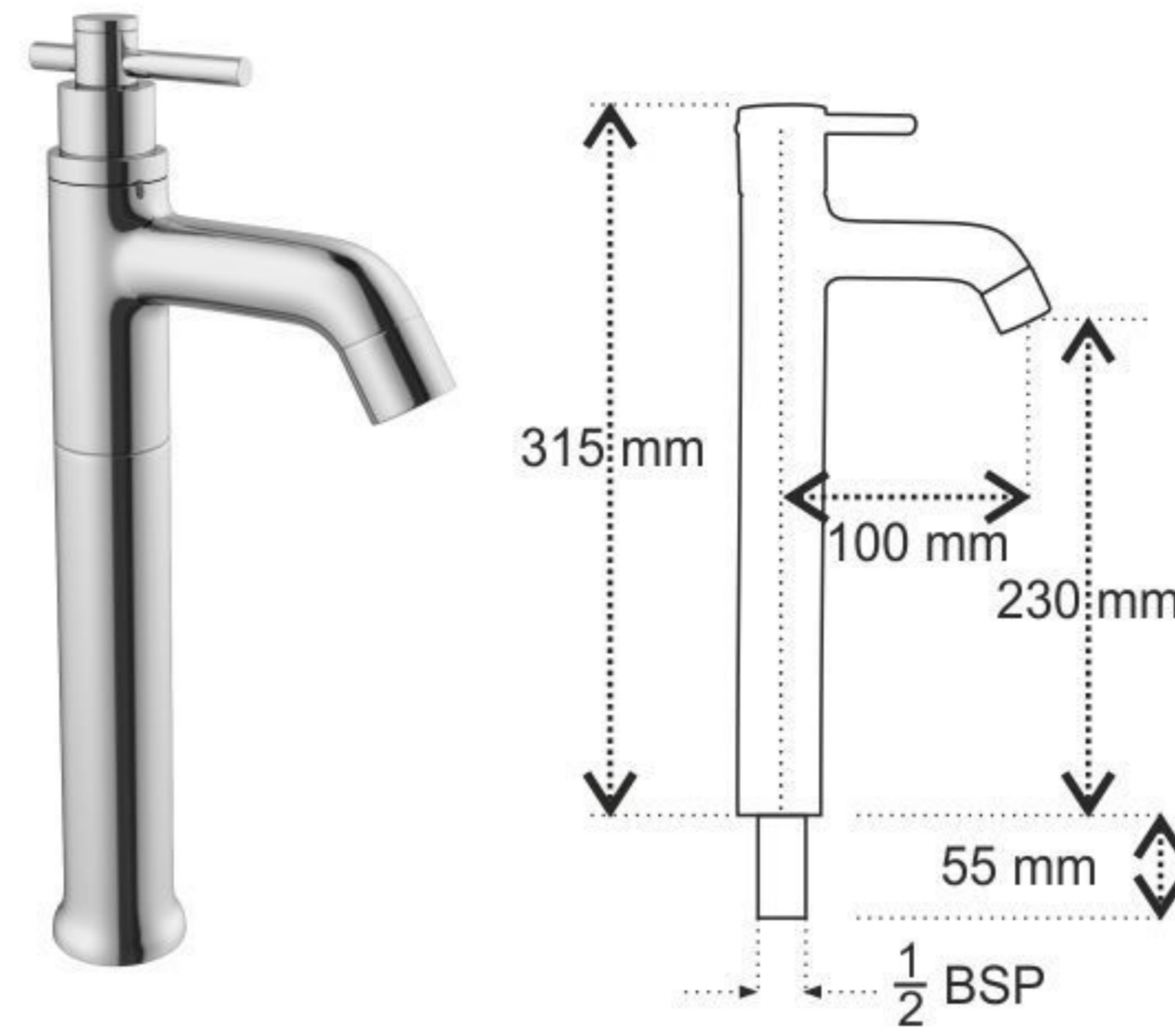
2826_Pillar Cock with Extension Body (Table Mounted)
