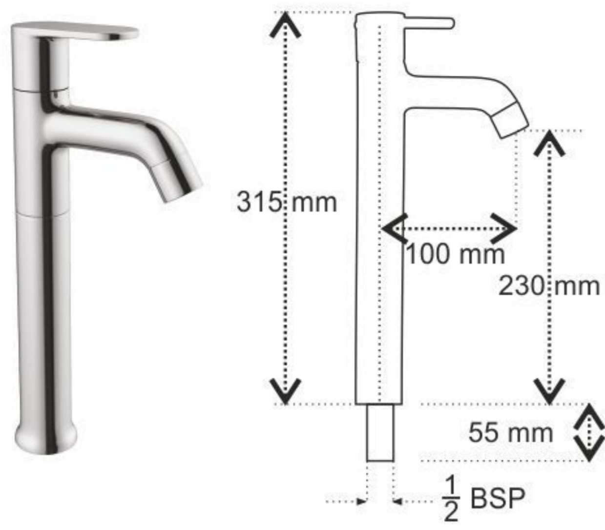
5226_Pillar Cock with Extension Body (Table Mounted)
