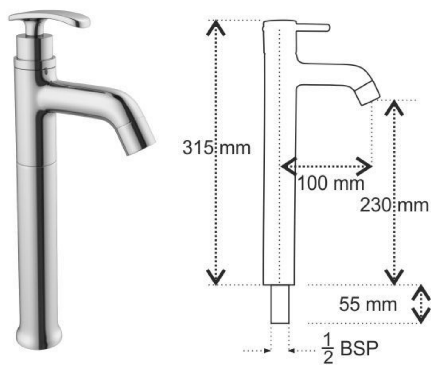
1326_Pillar Cock with Extension Body (Table Mounted)
